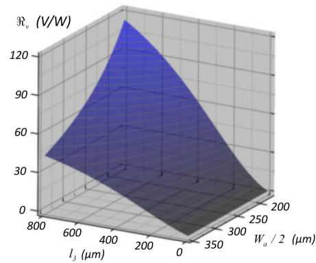
Figure 3. Sensitivity of the sensor as a function of l_3 and W_d/2 .
