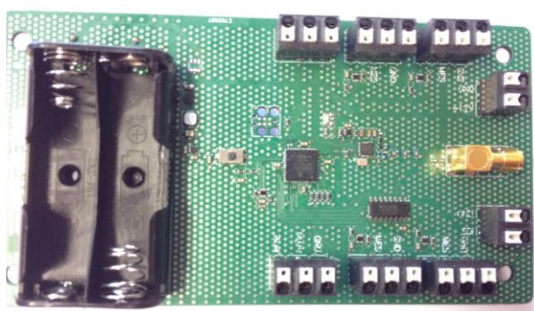
Figure 26. Photo of the electronic board produced
