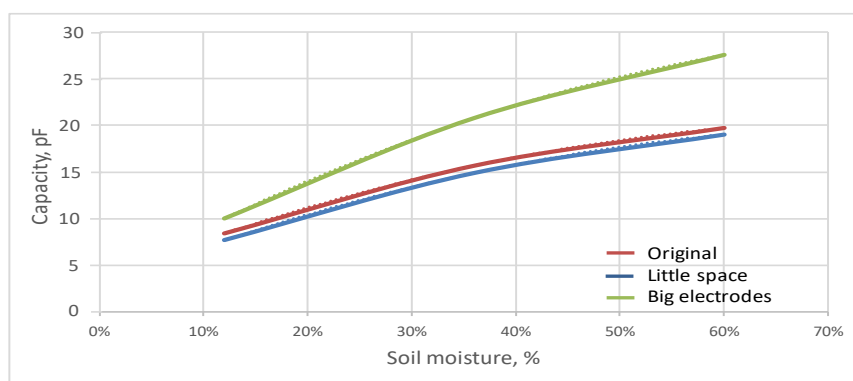
Figure 4. Capacity of different-sized electrodes as a function of moisture
