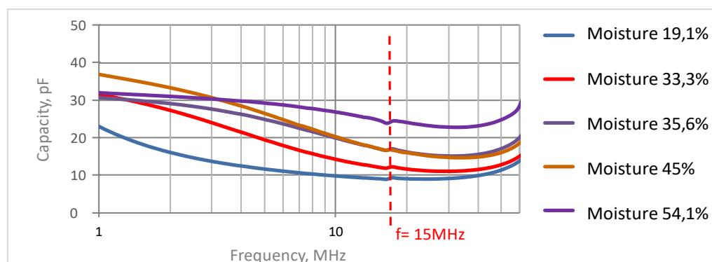
Figure 10. Sensor capacity as a function of the frequency
