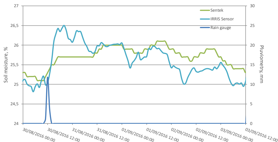
Figure 29. Sensor results compared with the Sentek sensor in a corn field
