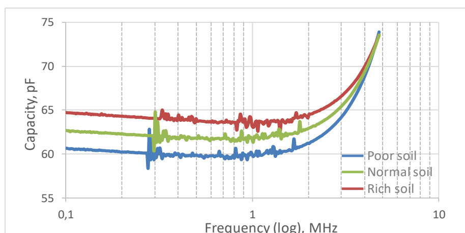
Figure 11. Sensor capacity as a function of the frequency for different levels of salinity
