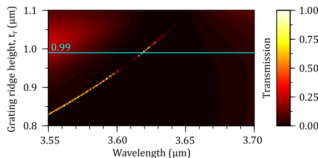
FIG. 3. Transmission spectrum as a function of the grating ridge height t_r . The light blue line corresponds to the case t_r = 0.99 \mu\text{m} , taken as reference for the rest of the study. The fixed device parameters are as follows: t_s = 0.22 \mu\text{m} , \Lambda = 1.255 \mu\text{m} and f\Lambda = 321.3 \text{ nm} .
