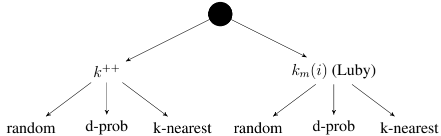
Figure 3: Representation of six different VNS heuristics defined by the mutator number sequence used and the neighborhood growth method used.
