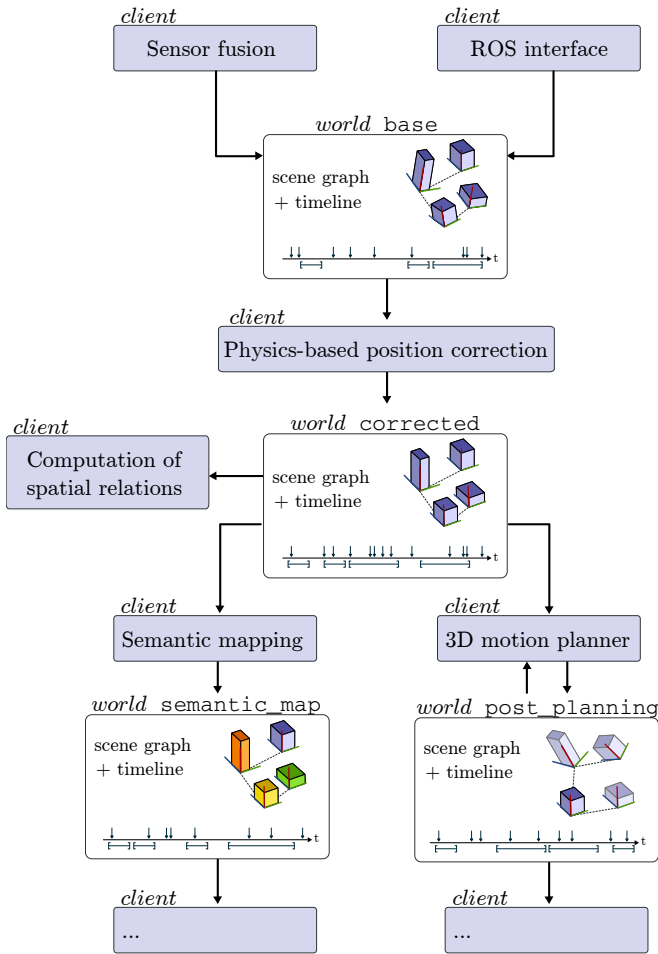
Fig. 1. Schema of a possible UNDERWORLDS network: eight clients (user-written & architecture specific; in blue) are sharing environment models through four independent worlds (made from joint spatial and temporal models). This architecture enables successive and modular refinement of the models ( cascading situation assessment ), effectively adapted to each client’s needs.
