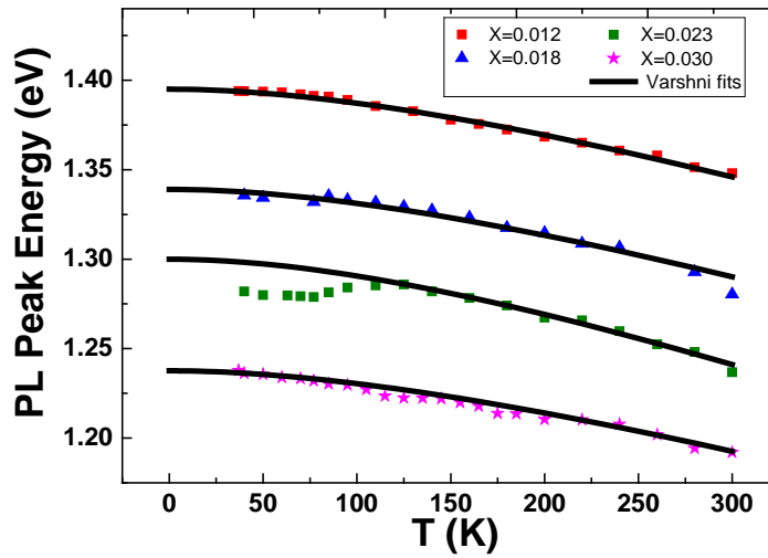
Figure 3 Temperature dependence of PL peak energy for the samples with various bismuth contents. Solid lines represent Varshni's fit.
