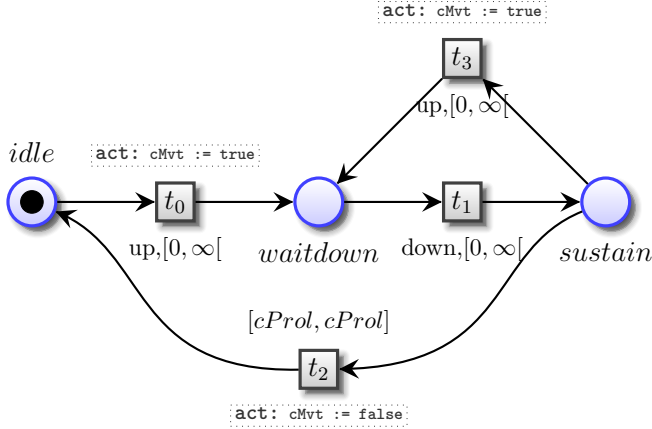
Fig. 3: CP_MON behavior
