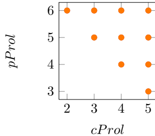
Fig. 5: Configurations for which DETECT is satisfied.
