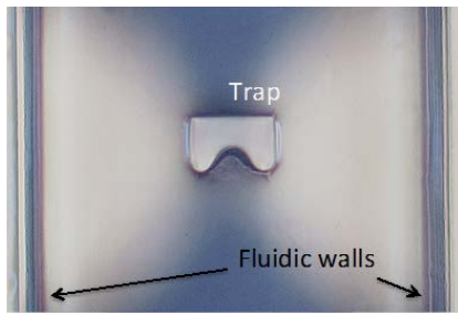
Fig. 2. Photography of the unloaded microwave sensor dedicated to single particle measurement.
