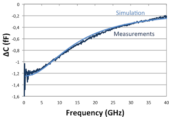
Fig. 3. Simulated and measured capacitive contrasts of a polystyrene bead with a diameter of 10\ \mu\text{m} on a capacitive gap of 10\ \mu\text{m} , in DI water.
