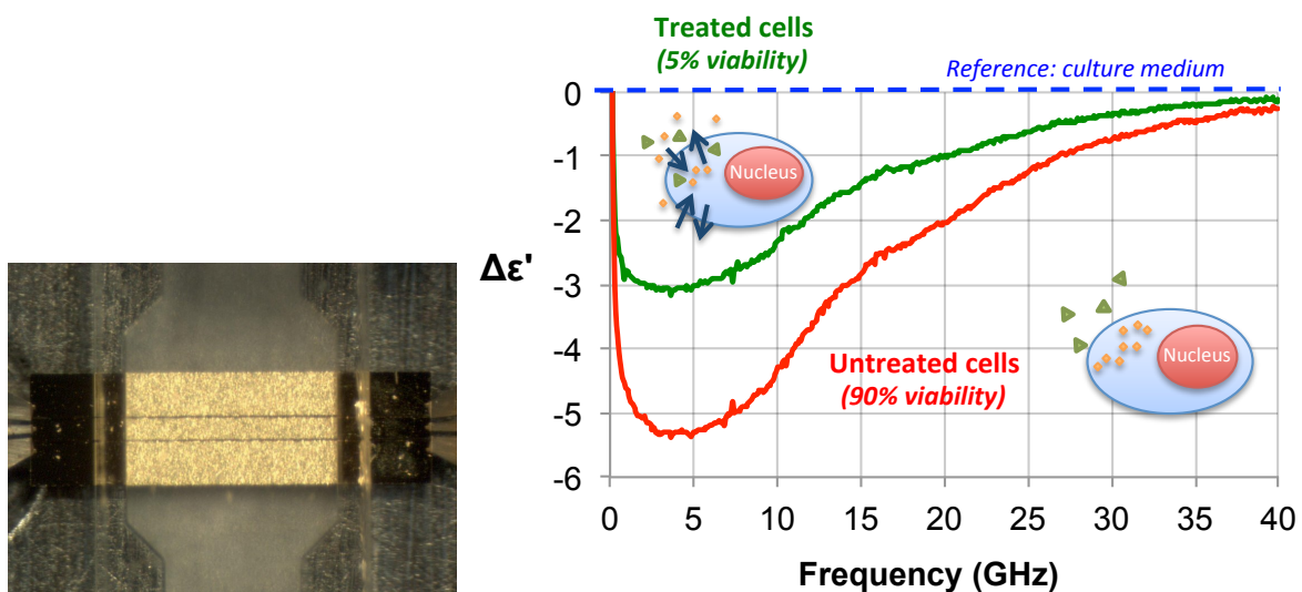
Figure 9. Picture of a coplanar waveguide loaded with DOHH-2 cells in suspension at the concentration of 100 Million cells/ml ; dielectric contrast of treated and untreated cells with saponin for membrane permeabilization [47].
