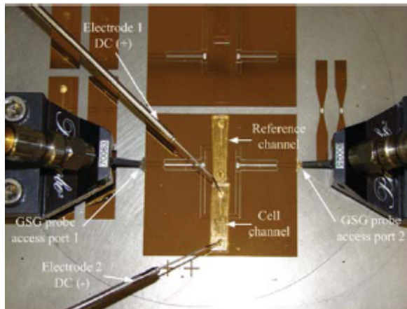
Figure 8. RF interferometer evaluated for yeast cells viability in de-ionized water [44].
