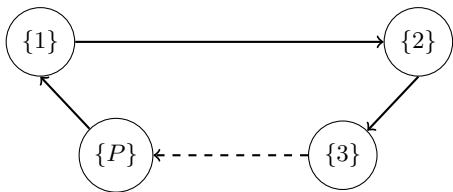
Fig. 1: An automaton for round-robin protocols.
