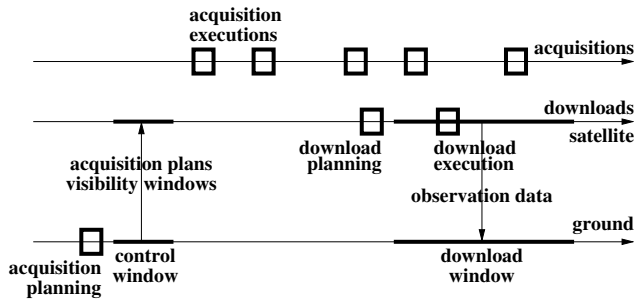
Figure 1: Decision-making organization.
