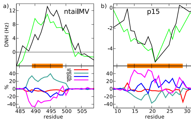
Figure 3: Experimental (black) and hybrid building model (green) N-HN RDCs for two fragments of (a top) ntailMV and (b top) p15. Fragments highlighted in orange were considered partially structured and built using the TRS strategy. In bottom panels, the percentage of enrichment of secondary structure classes present in the ensemble built with the hybrid strategy compared with that built with the SRS strategy. Secondary structure classes were identified using definitions in related work (Ozenne et al., 2012b). Concretely, [\beta S : -100 > \phi; -120 > \psi > 50] , [\beta P : 0 > \phi > -100; -120 > \psi > 50] , [\alpha R : 0 > \phi; 50 > \psi > -120] , [\alpha L : \phi > 0] .
