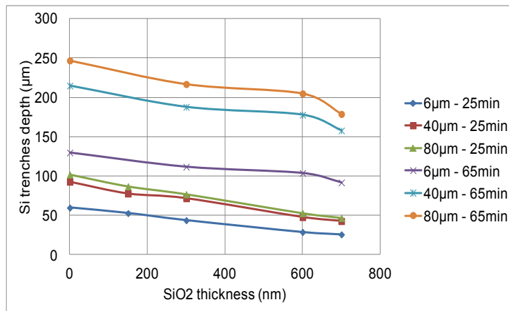
Figure 10: Silicon depth variations versus SiO_2 mask thickness for 25 min and 65 min etching times and different trench widths ( 6\ \mu\text{m} , 40\ \mu\text{m} , 80\ \mu\text{m} )
