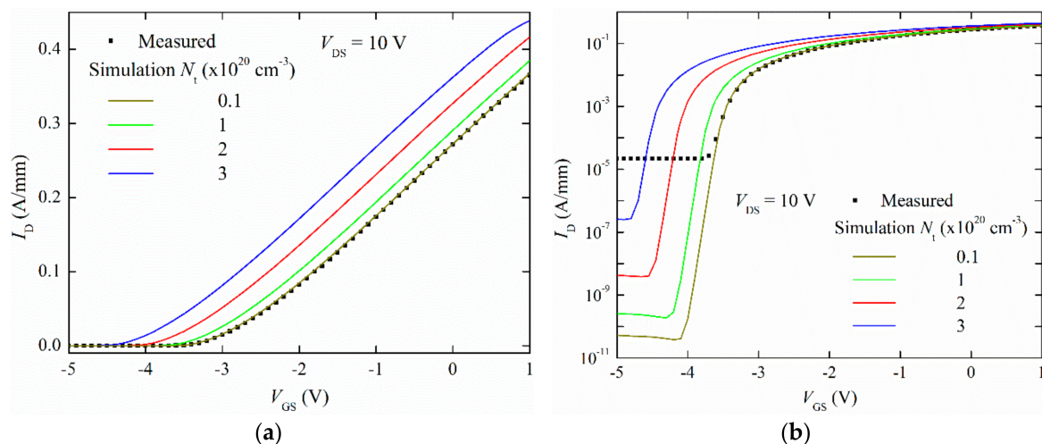
Figure 2. Measured (symbols) and simulated (lines) transfer characteristics for the AlGa N /GaN HEMT, for different traps concentration, with drain current in (a) linear scale and (b) logarithmic scale; V_{DS} = 10 V.
