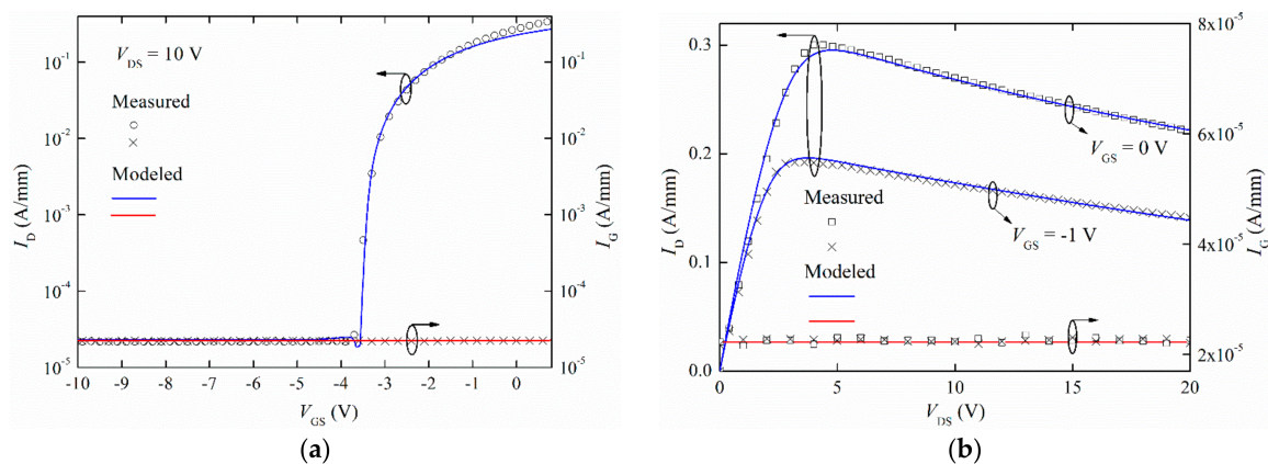
Figure 8. Measured (symbols) and modeled (lines) (a) transfer characteristic in saturation regime (left axis, with V_{DS} = 10 V) and corresponding gate current (right axis), in logarithmic scale, and (b) output characteristics (left axis) and corresponding gate current (right axis), at different gate voltages: V_{GS} = -1 and 0 V.
