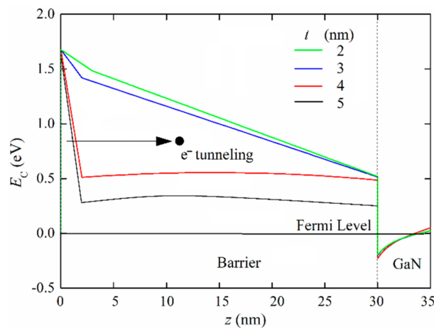
Figure 3. Conduction band energy minimum vs. depth under the gate, when varying the thickness of the donor traps layer beneath the gate: t = 2, 3, 4, and 5 nm.
