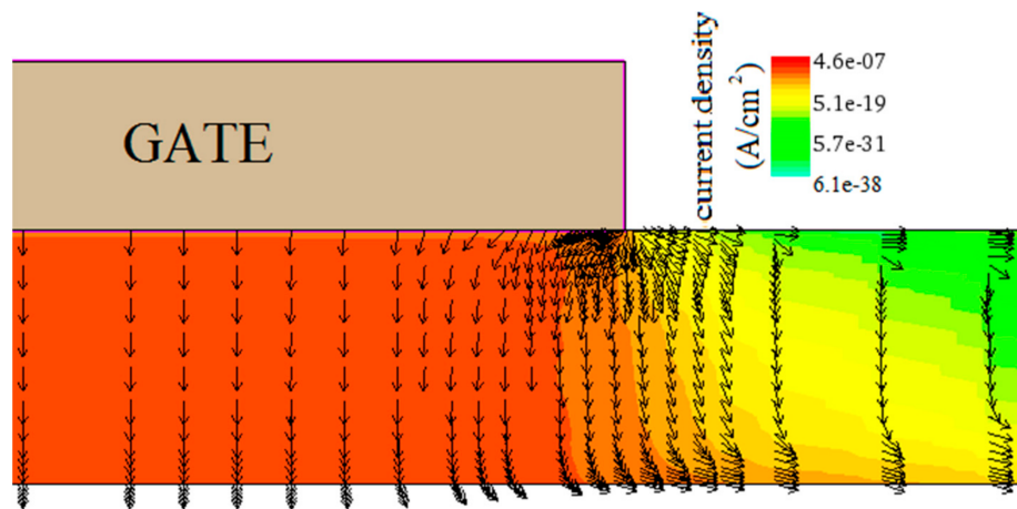
Figure 7. Current density flow through the barrier; V_{GS} = -5 V and V_{DS} = 10 V.
