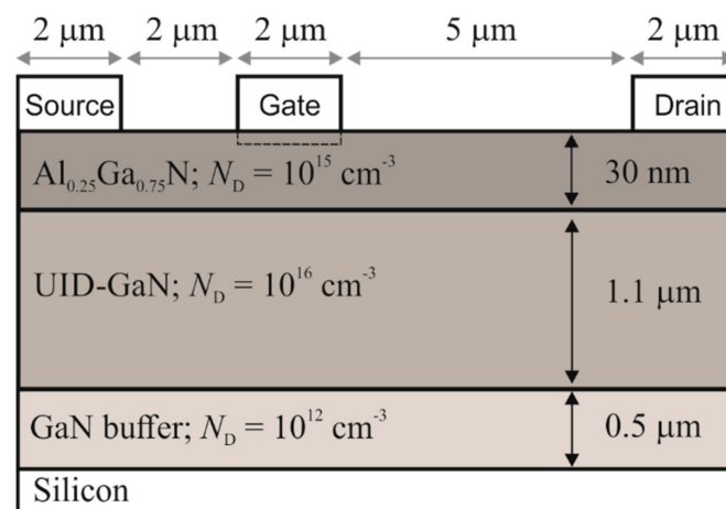
Figure 1. Simulated AlGaIn/GaN HEMT. Below the gate, the donor trap layer is indicated with dashed lines.
