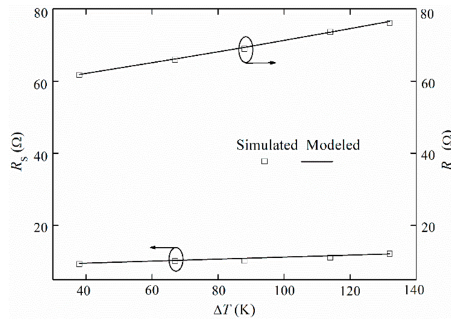
Figure 6. Numerical (symbols) and modeled (lines) R_S (left axis) and R_D (right axis) against device temperature increment.
