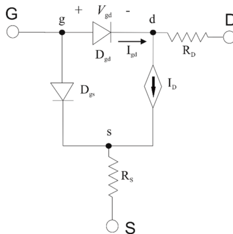
Figure 5. HEMT large signal equivalent circuit.
