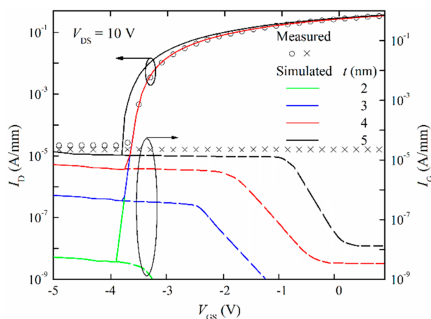
Figure 4. Measured (circles) and simulated (solid lines) transfer characteristics in logarithmic scale (left axis), and corresponding measured (crosses) and simulated (dashed lines) gate current (right axis).
