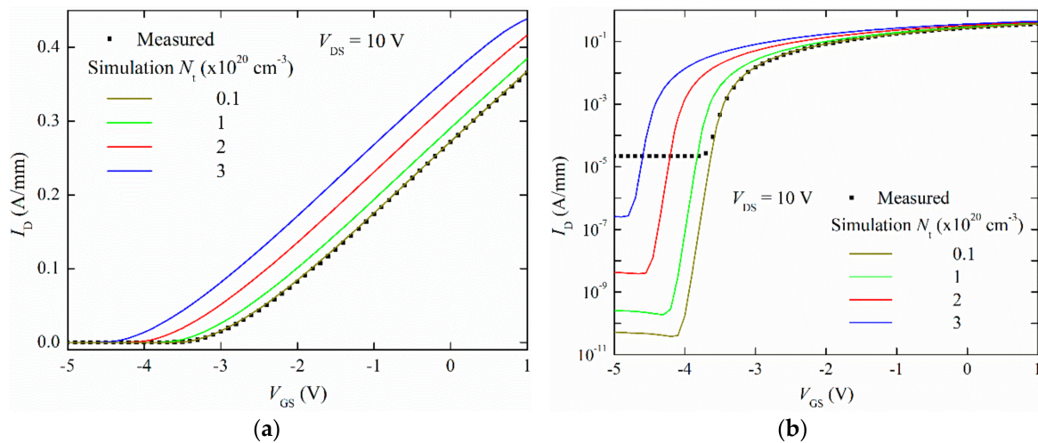
Figure 2. Measured (symbols) and simulated (lines) transfer characteristics for the AlGaIn/GaN HEMT, for different traps concentration, with drain current in (a) linear scale and (b) logarithmic scale; V_{DS} = 10 \text{ V} .
