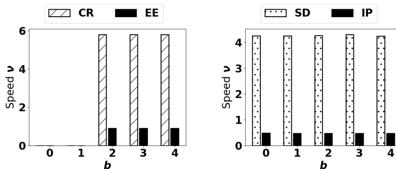
(a) Domains having dead ends (CR and EE)
