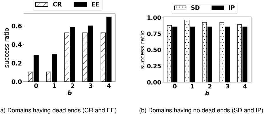
Figure 2. Success ratio (number of successful jobs/ total number of jobs) for different values of search breadth b . CR = Chargeable Robot, EE = Explorable Environment, SD = Spring Door, IP = Industrial Plant.
