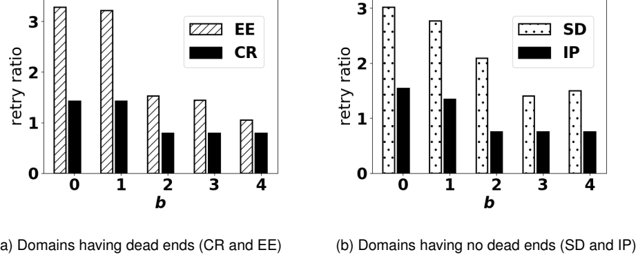
Figure 3. Retry ratio (number of retries / total number of jobs) for different values of search breadth b . CR = Chargeable Robot, EE = Explorable Environment, SD = Spring Door, IP = Industrial Plant.
