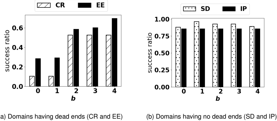
Figure 2. Success ratio (number of successful jobs/ total number of jobs) for different values of search breadth b . CR = Chargeable Robot, EE = Explorable Environment, SD = Spring Door, IP = Industrial Plant.
