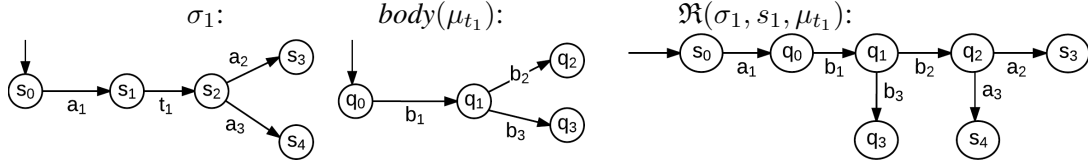
Figure 5. Three IOAs: \sigma_1 , body(\mu_{t_1}) , and \Re(\sigma_1, s_1, \mu_{t_1}) . Note that a_1 b_1 b_2 a_2 is a closed path of \Re(\sigma_1, s_1, \mu_{t_1}) , with proj_{\sigma_1}(a_1 b_1 b_2 a_2) = a_1 t_1 a_2 and proj_{\mu_t}(a_1 b_1 b_2 a_2) = b_1 b_2 .
