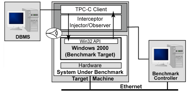
Figure 1. Experimental set-up
