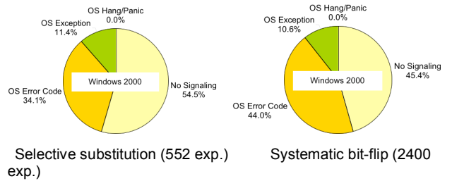
Figure 4: Sensitivity to corruption technique
