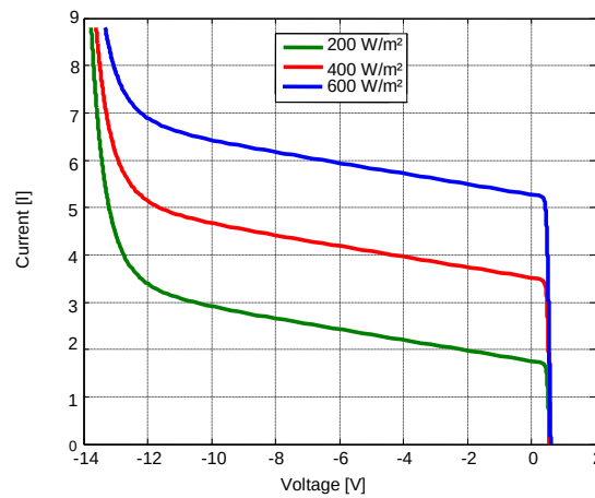
Fig. 3 : The I-V curves for different illuminations
