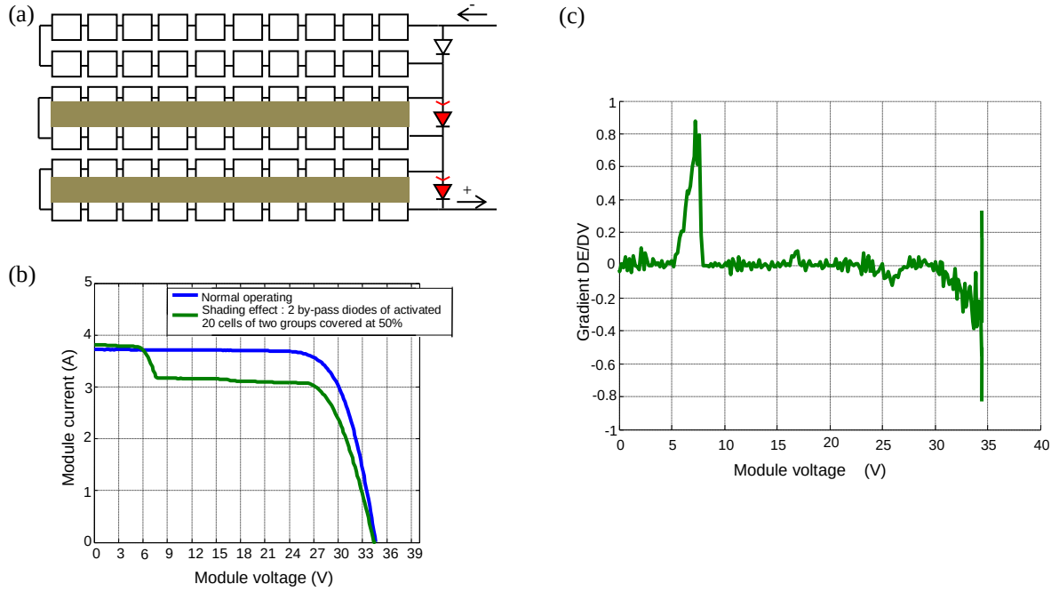
Fig. 9 : Shading set 6 – (a) the shadow scenario, (b) the impact of the shadow over the I-V curve and (c) the results from the proposed detection method.
