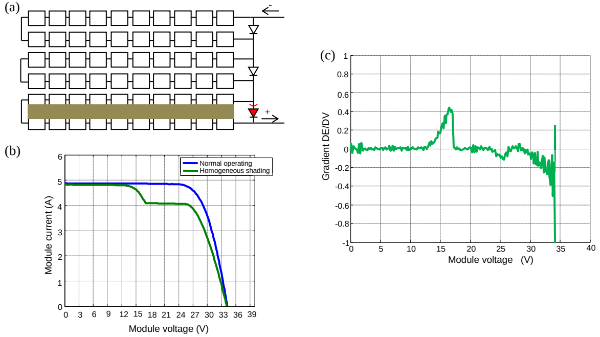
Fig. 7 : Shading set 3 – (a) the shadow shape, (b) the impact of the shadow over the I-V curve and (c) the result from the detection method
