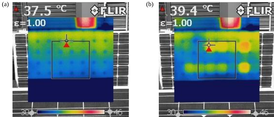
Fig. 1 : IR camera test on PV module in open circuit (a) and in short circuit (b)
