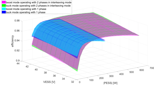
Fig. 3. Experimental efficiency for all the configurations of the MISB converter
