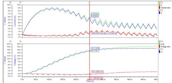
Fig. 13: Capacitor voltage of boost converter model using VHDL code from HiLeS platform.
