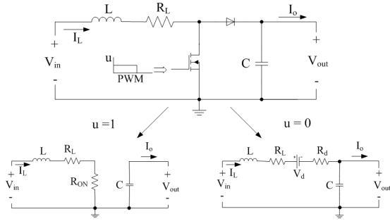
Fig. 6: Boost converter.
