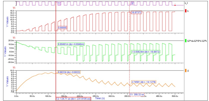
Fig. 12: Inductor current of boost converter model using VHDL code from HiLeS platform.
