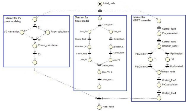
Fig. 11: Partial general control Petri net of the PV system model.
