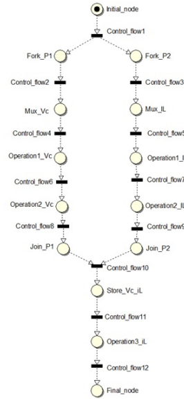
Fig. 8: Partial control Petri net of boost converter model.
