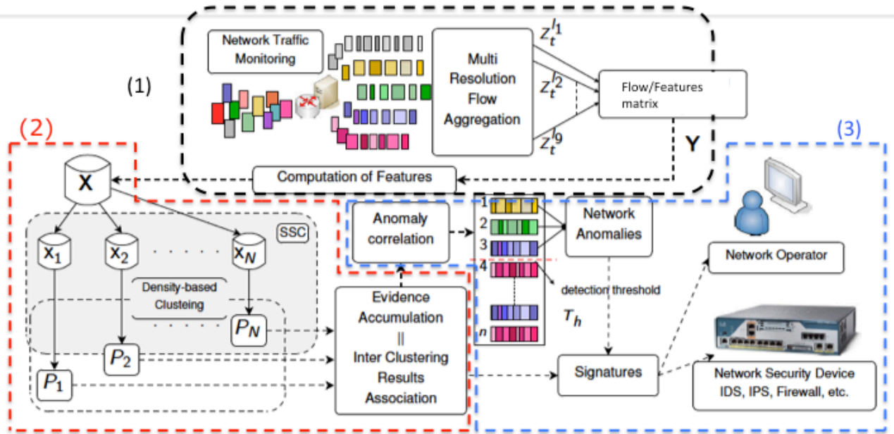
Figure 3: High-level description of the Unsupervised network Anomaly Detection System
