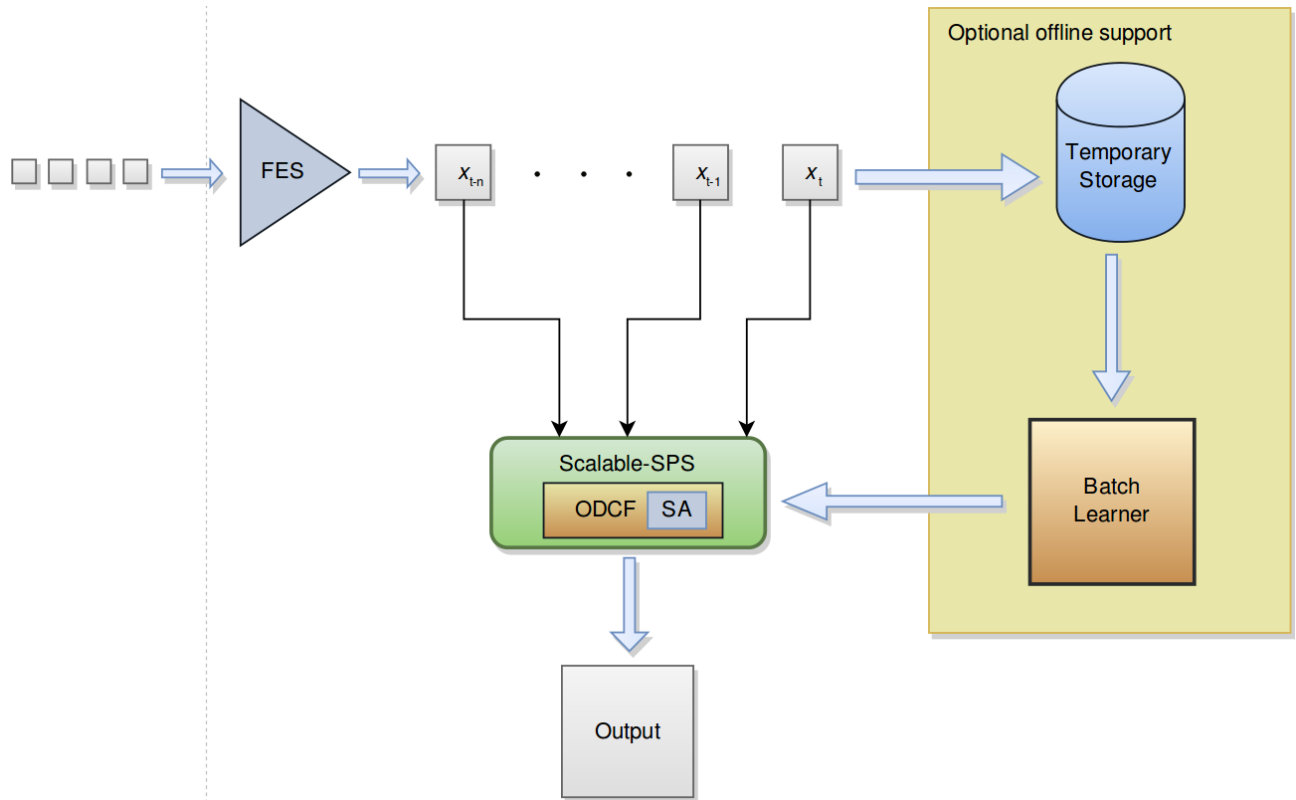
Figure 2: Traffic Pattern Evolution Subsystem Architecture
