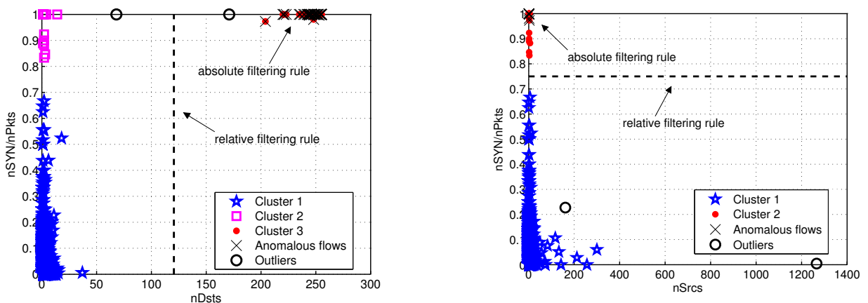
Figure 5: SYN network scan
