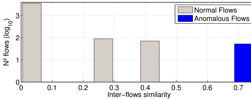
Figure 4: Detecting a distributed SYN network scan using S
