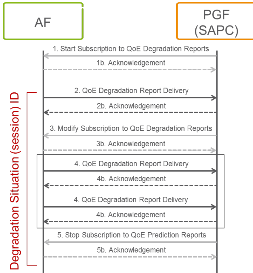
Figure 18: Standard dialogue between AF and PGF
