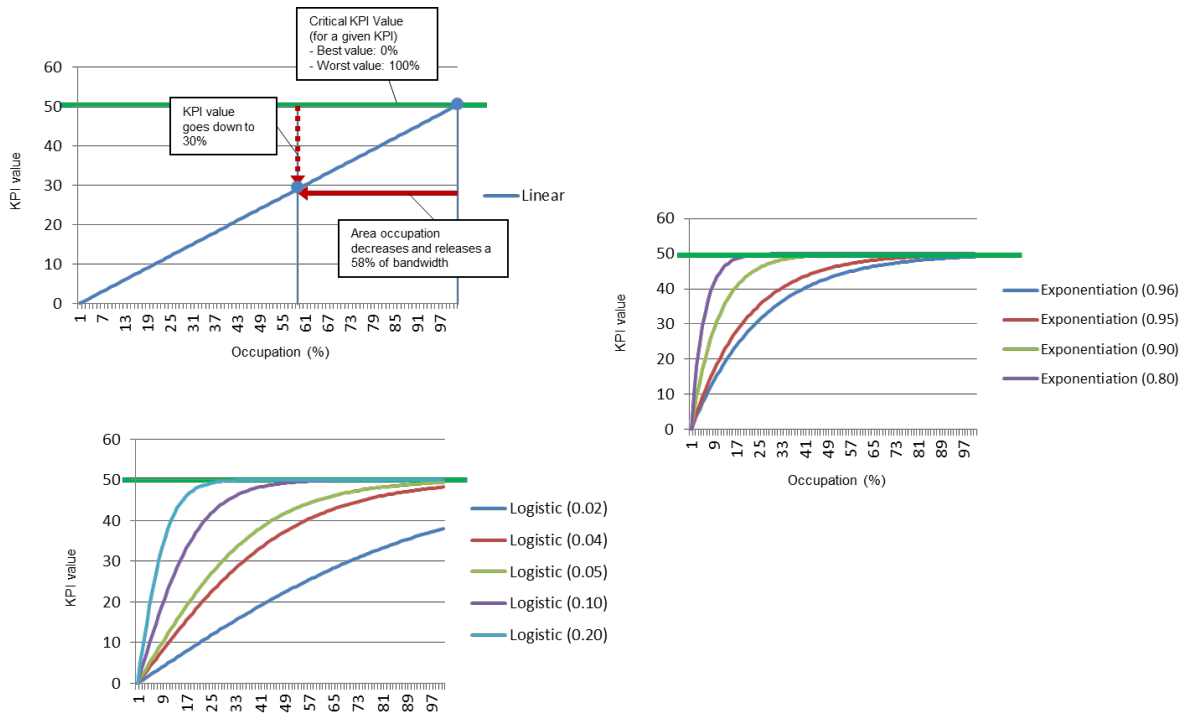
Figure 14: Function modelling the bandwidth release and the KPI gain (Linear, Exponentiation, and Logistic)
