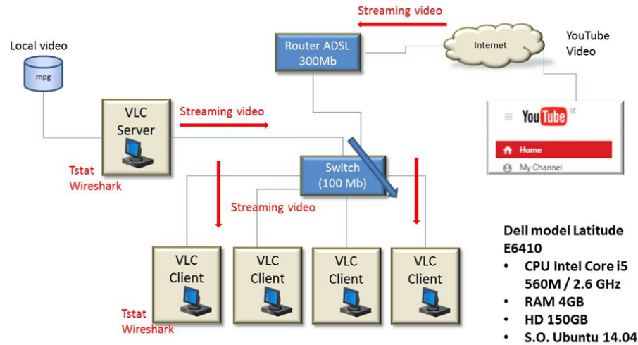
Figure 9: VLC test-bed
