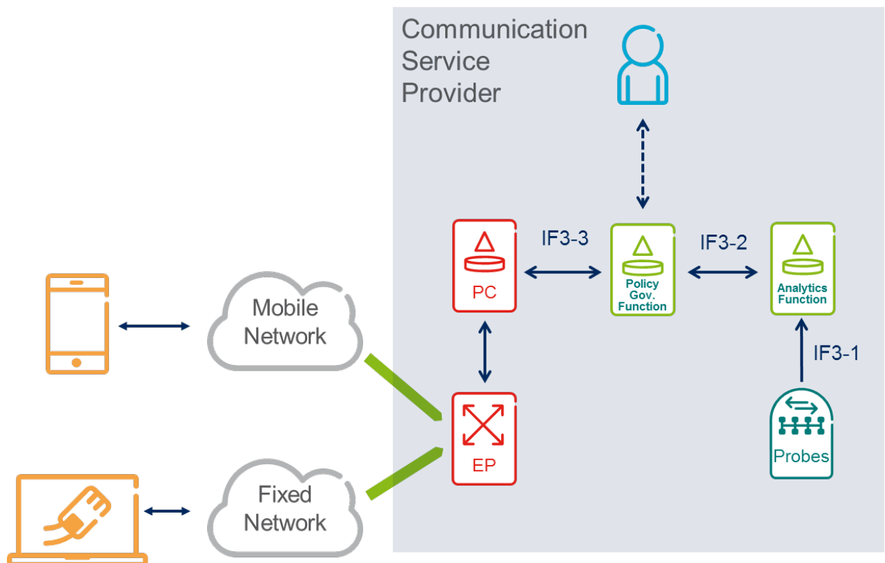
Figure 10: UC #3 System Architecture
