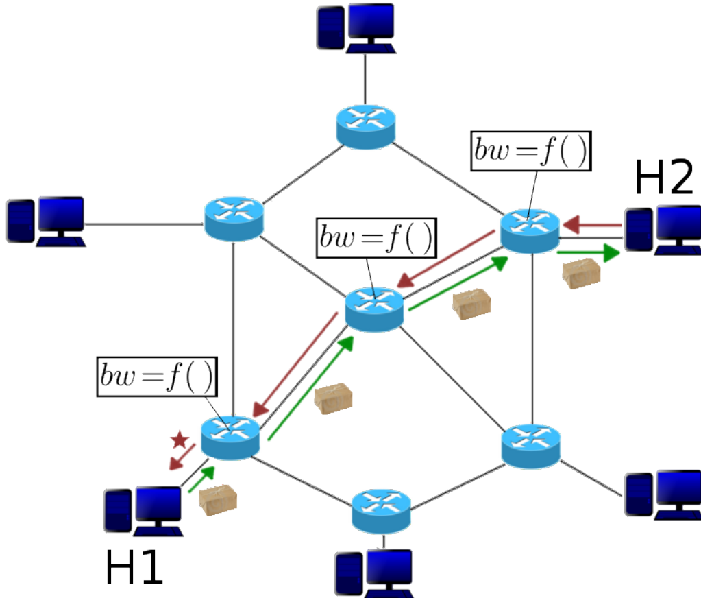
Figure 6: An example of how EERC protocols work.
