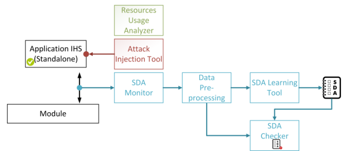
Figure 6. Prototype Architecture
