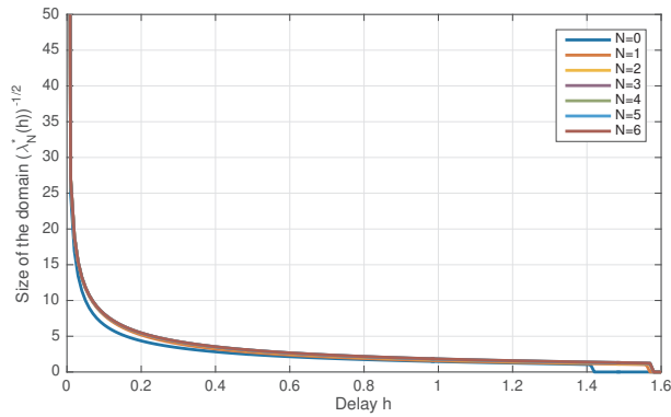
Fig. 1. Evolution of (\lambda_N^*(h))^{-1/2} with respect to h in [0, 1.6] , for N = 0 to 6.
