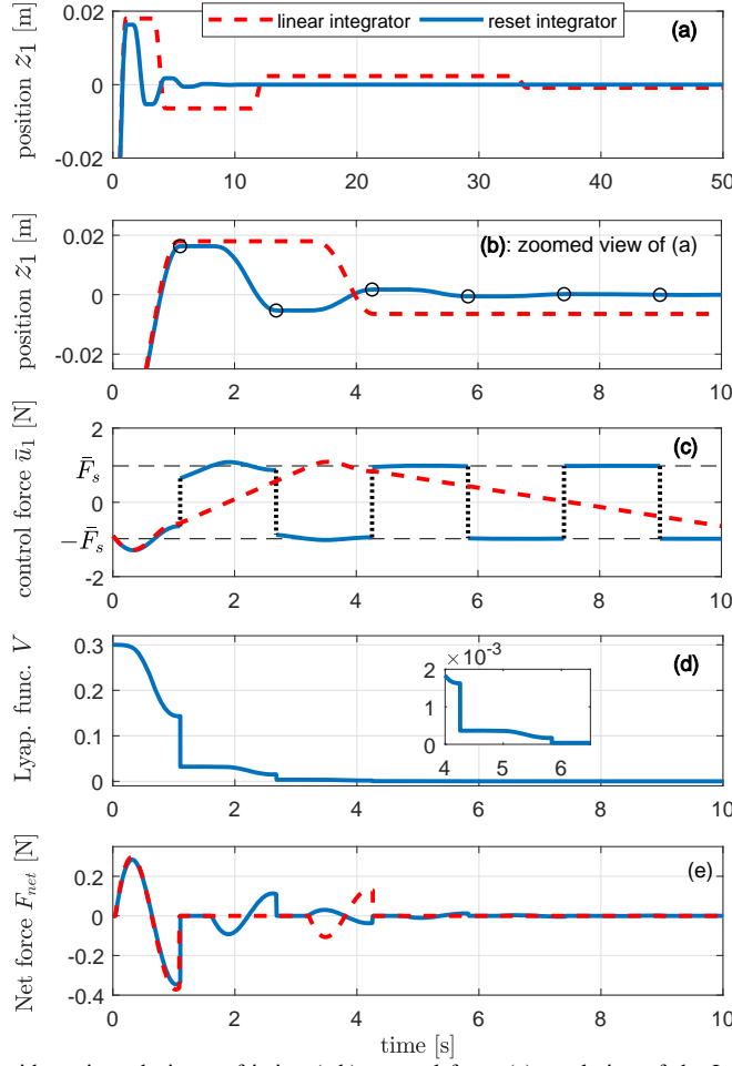
Fig. 3. Simulated position response with static and viscous friction (a,b), control force (c), evolution of the Lyapunov-like function (d), and net force acting on the system (e).
