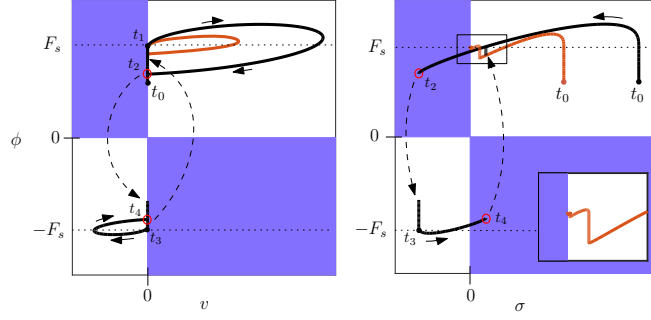
Fig. 2. Phase portraits corresponding to the response in Fig. 1 (black). The jump criteria \phi v \leq 0 (left) and \phi \sigma \leq 0 (right) are indicated in blue. A state jump (from the red circles) follows the dashed arrows. The red line corresponds to a different solution without overshoot, which then comes close to the jump set but never enters it, as designed (see the zoomed box). For clarity, we did not show the condition |\phi \sigma| \geq \varepsilon in the figure. See Fig. 1 for times t_0, \dots, t_4 .
