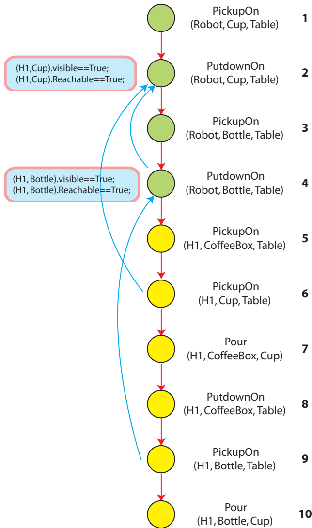
Figure 5: An example of a plan for coffee making scenario.
