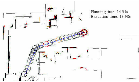
Figure 5: Execution of the original planned path by the Nomad
