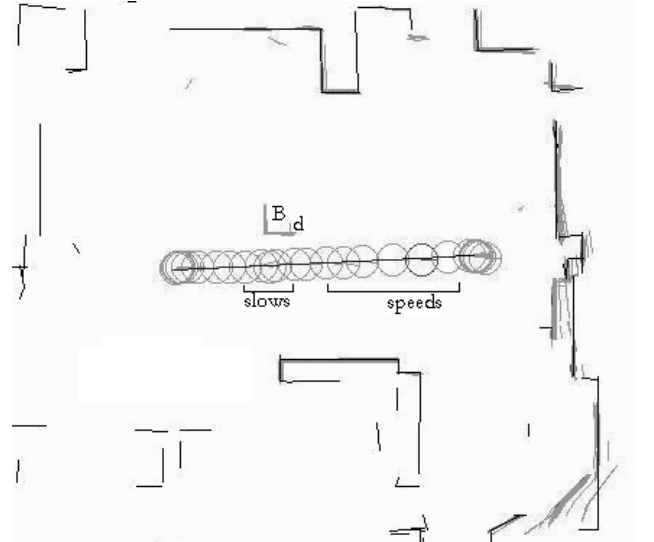
Figure 30: Unreduced path executed by the Nomad XR4000. The vertex d of the new box shaped object B forces a slow down near it.
