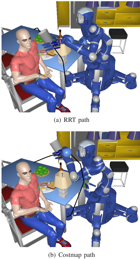
Fig. 7. A complete object hand over example scenario. The robot has the object in its hand. The human is sitting on a chair looking away from the robot. While the motion planned with a standard planner does not consider the presence of the human, the one planned by taking into account the three constraints generates a comfortable motion. By following this path the robot stays as visible as possible, as sufficiently far as possible and the object is comfortable to reach by the human.
