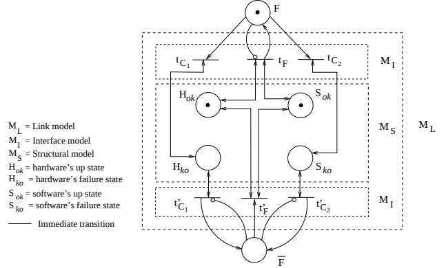
Figure 5. Two series components
