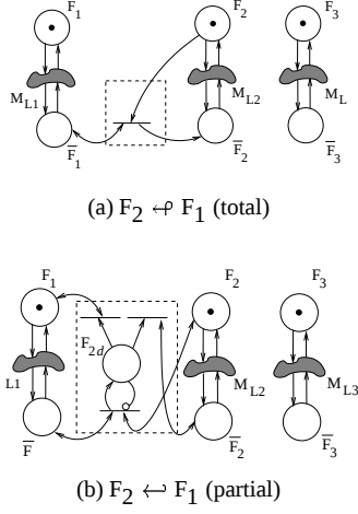
Figure 4. Functional dependencies
