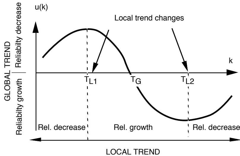
Fig. 3 Laplace factor and reliability evolution
