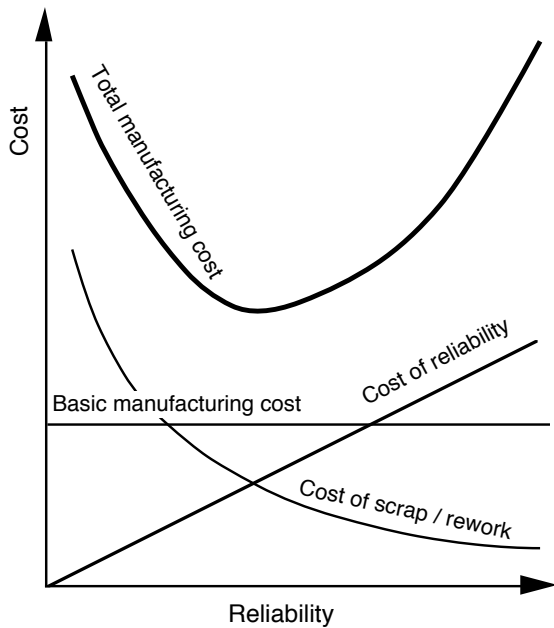
Fig. 1 Cost and reliability for the supplier
