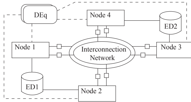
Fig. 2. MMS reference architecture
