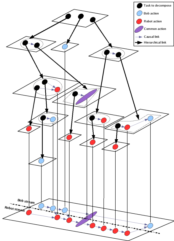
Fig. 1. HATP plan structure: the Refinement Tree and the Time Projection
