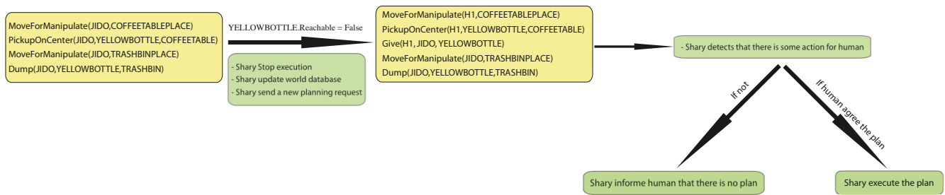
Figure 6: Example 2 (In difficulty ask Help, if possible): clean-up task execution: The yellow square represents HATP plan's, the green square represent decision and action. The first plan failed due to robot inability to take the bottle (even when it has perceived it), then Shary asks a new feasible plan. HATP finds a plan with a higher cost and two streams and where the person is requested to participate by giving the bottle to Jido. Shary asks human if he agrees with the now plan. if the answer is positive, Shary starts execution of plan else it informs the human that there is no plan.
