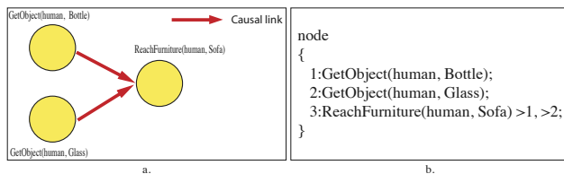
Figure 4: HATP goal description. : a.) graphical representation. b.) textual representation with > representing the preference constraints
