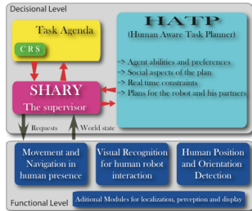
Figure 2: A control Architecture for a proactive robot assistant.
