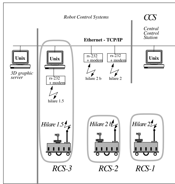
Figure 9. The experimental testbed
