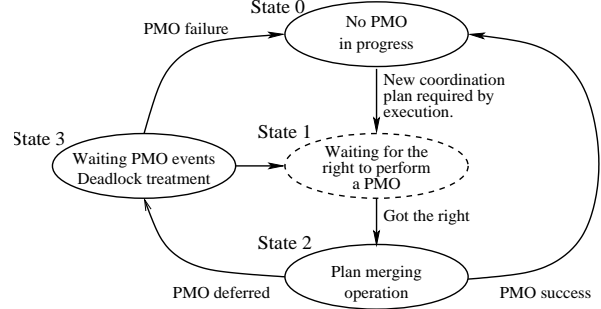
Figure 2: The Plan Merging Protocol.
