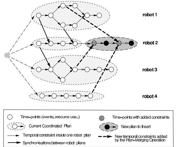
FIG. 4 – Robot 2 performs a PMO.
