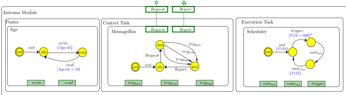
Figure 7: Antenna module implementing timing constraints using clocks.
