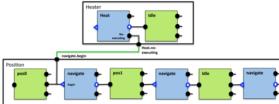
Figure 12: Example of modeling Timelines using BIP.
