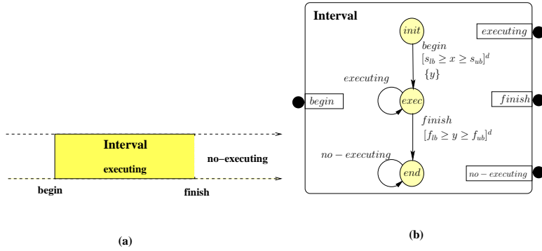
Figure 8: Modeling an interval (a) as a BIP atomic component (b).
