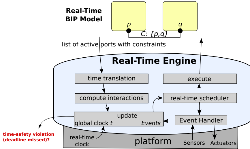
Figure 6: The real-time BIP engine.
