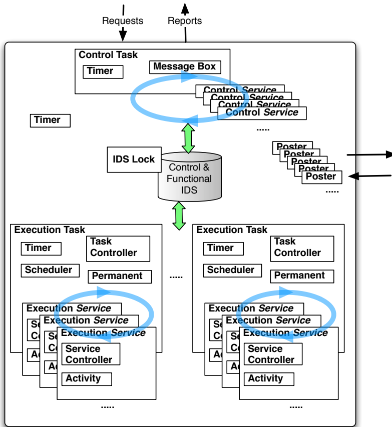
Figure 1: A G^{\text{en}}M module functional organization and its componentization prior to BIP modeling.
