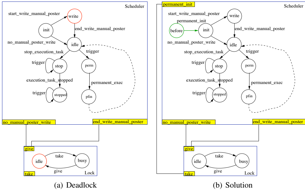
Figure 15: A deadlock (a) and its solution (b). In both figures the top component is a Scheduler and the bottom one is a Lock .
