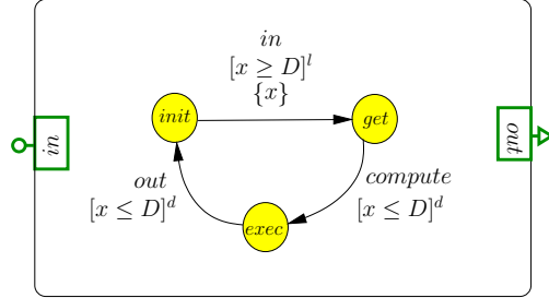
Figure 5: A timed BIP atomic component.
