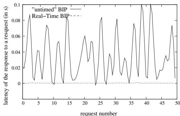
Figure 16: Comparison between real-time BIP and untimed (standard) BIP.
