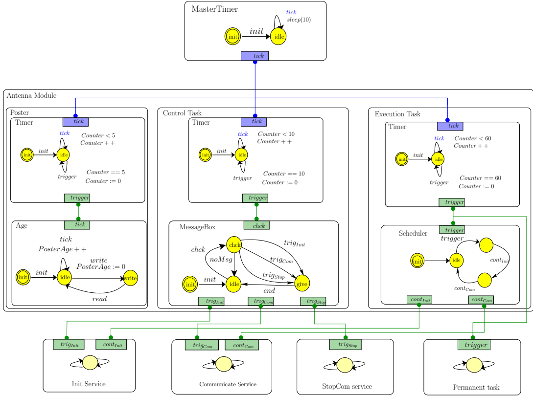
Figure 4: Antenna module implementing timing constraints using ticks.
