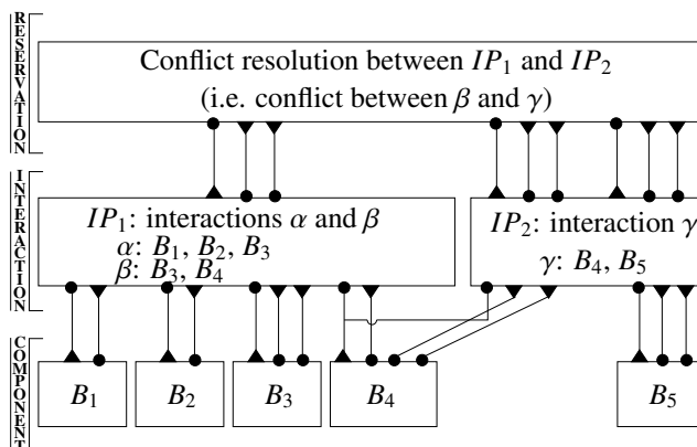
Figure 17: Send/Receive BIP model obtained from BIP-to-BIP transformations.
