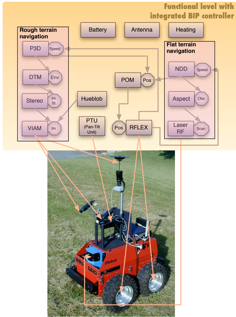
Figure 2: The functional modules of the Dala rover.
