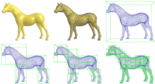
Fig. 2. The object mesh is uniformly sampled with a point set (top images). The point set is then partitioned using a kd-tree (bottom images).
