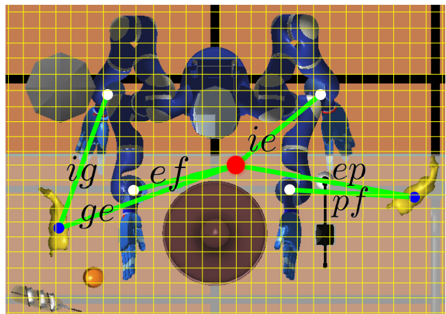
Fig. 6. Top view of a pick-and-place task showing the elementary distances to be minimized over a 3D grid in order compute the double grasp position (the center red circle)
