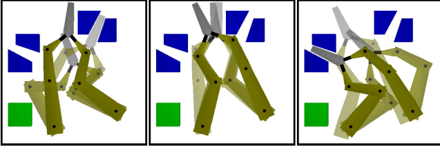
Fig. 5. Solution to problem B. The images show three parts of the solution path. The first part (left) corresponds to the sub-path between the initial configuration and the first singularity, which permits the reconfiguration of the left arm. The second one (middle) shows the sub-path to the second singularity (reconfiguration of right arm). The third sub-path (right) reaches the final configuration.
