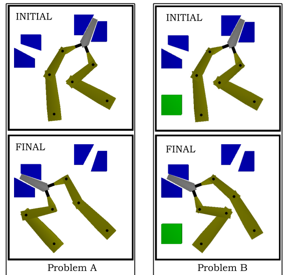
Fig. 1. Academic example of path planning problems for coordinated manipulation. The solution to problem B requires the reconfiguration (elbow up/elbow down) of both manipulators.
