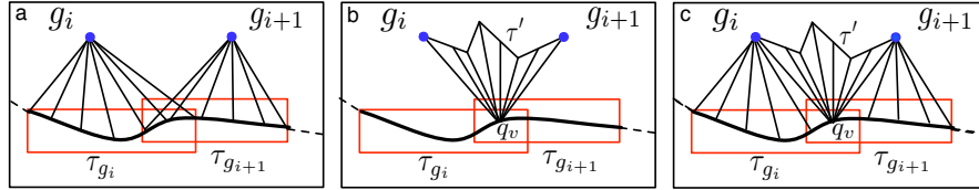
Fig. 6. A RCPV roadmap is a visibility deformation roadmap. (a) the visibility of the guardians gives first patches of ruled surfaces. (b) the RCPV roadmap property guarantees the visibility of a roadmap path connecting two guardians. (c) By construction, a global visibility deformation surface can be built.
