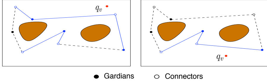
Fig. 5. Two examples of visible subroadmap from a given configuration q_v . On the left, the visible subroadmap is disconnected whereas it is connected on the right.
