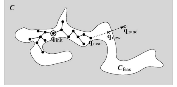
Fig. 2. Illustration of one expansion step of an RRT search tree. The tree tends to cover C_{feas} : the feasible subset of the configuration space C .
