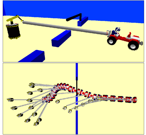
Figure 7: Non-holonomic car tracks a pipe coordinating with a mobile manipulator.
