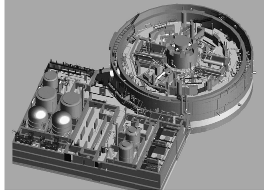
Figure 1: Auxiliaries building (level 5) and reactor building (level 6) of a N4 nuclear power plant (EDF, Engineering and Construction Division).
