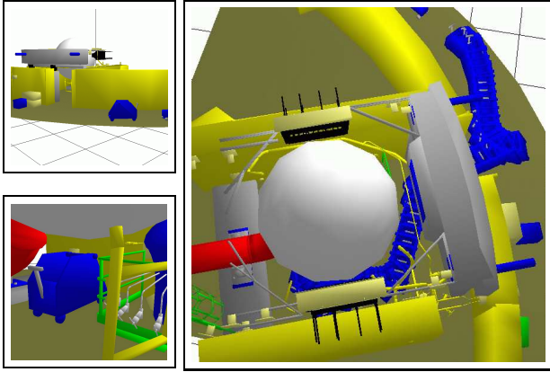
Figure 4: Nonholonomic cart in a steam generator of a nuclear plant (model provided by EDF)
