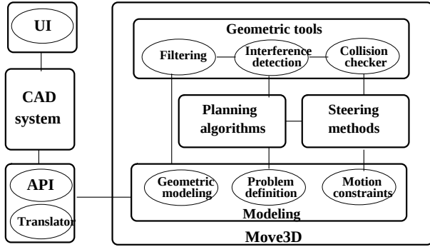
Figure 3: Architecture of Move3d
