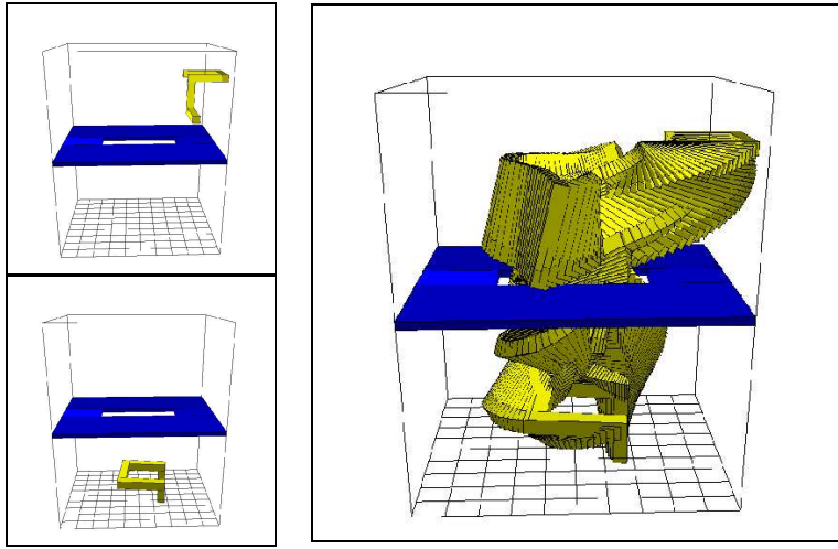
Figure 4: A solution path for the 6-dof puzzle problem presented in [12].
