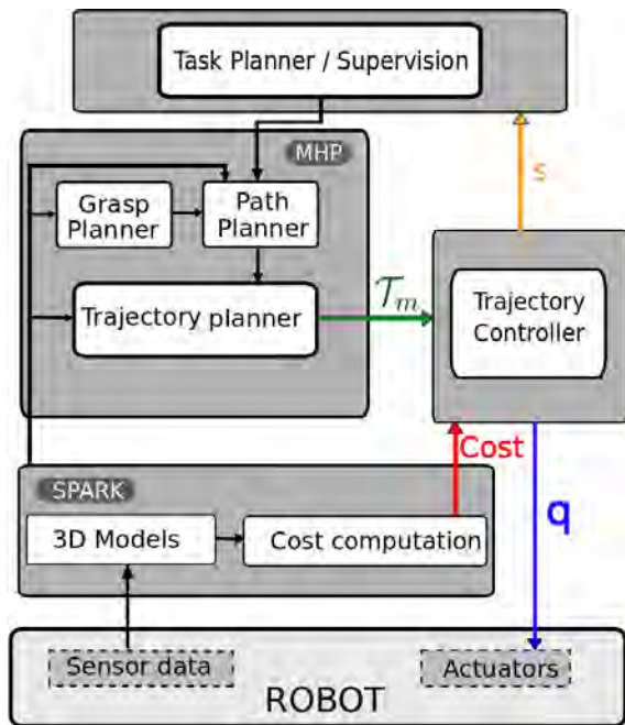
Figure 1: Software Architecture of the robot for HRI manipulation. T_m is the main trajectory calculated initially by MHP(Motion in Human Presence). The controller takes also cost maps from SPARK. The controller sends control signals in joint( q in the figure) to the servo system, and during the execution, the controller sends the state of the controller ( s ) to the supervisor
