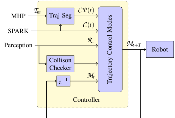
Figure 4: Input and output of the controller. \mathcal{T}_m is the trajectory computed by MHP, it is then segmented into control primitives ( \mathcal{CP}(t) ). Traj Seg represents trajectory segmentation . C(t) are the cost values. \mathcal{R} represents the transformation matrices, giving the position of the target and of the robot. \mathcal{M}_t is the current state of the robot, \mathcal{M}_{t+T} is desired motion condition for the next control cycle. z^{-1} represents delay of a control cycle.
