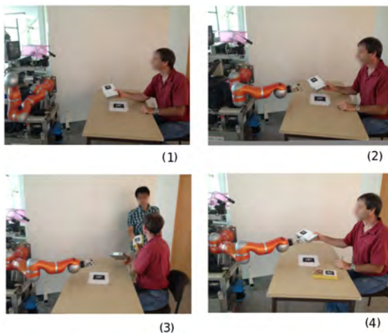
Figure 12: (1): The controller is given the task of receiving the object from human. It tracks the first segment in the robot frame. (2): The object is moving and the robot tracks a target. (3): Human is distracted by another human and the task is suspended. (4): Human returns to the task, and the robot resumes the task and grasps the object.
