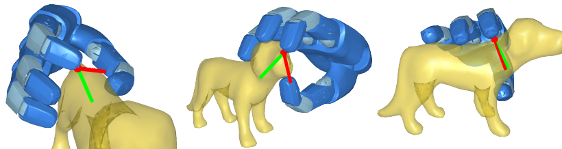
Figure 7: The major axis of the forefinger force ellipsoid for different contacts (red lines) and the normals of the contacts (green lines). It is preferable to have contact with a limited angle between these two lines (right image) rather than large one (left images) to reduce of contact slipping if the finger closing strategy does not use grasping force optimization and control.
