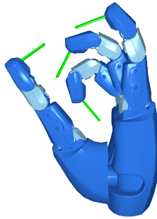
Figure 6: The major axes of each finger force ellipsoid are drawn as green lines. They are used to remove candidate contacts according to their normal.
