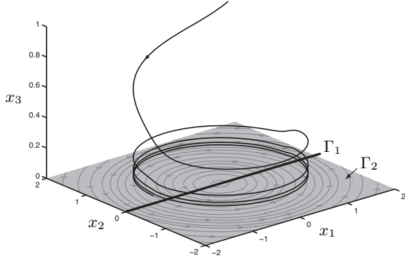
Figure 3: Example 4.6: \Gamma_1 is globally attractive relative to \Gamma_2 , \Gamma_2 is globally asymptotically stable, and yet \Gamma_1 is not attractive.
