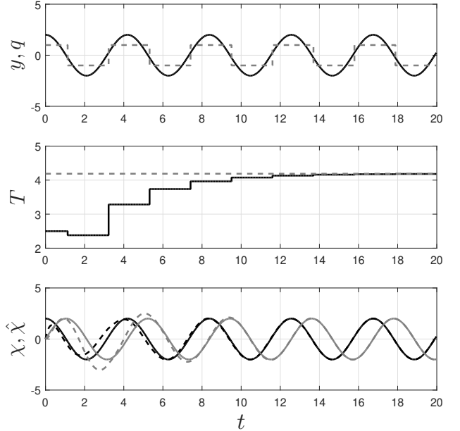
Figure 5: Top Graph: time histories of the function y generated by (18) and of the state q(t, k) , solid and dashed lines, respectively. Middle Graph: time histories of the estimate T(t, k) , converging to the correct value of the period of oscillation 2\pi/\omega . Bottom Graph: time histories of \hat{\chi}_1(t, k) (dark) and \hat{\chi}_2(t, k) (gray), solid lines, converging to the actual states \chi_1(t, k) and \chi_2(t, k) , dashed lines.
