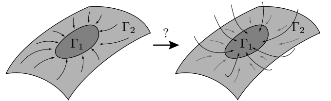
Figure 2: Illustration of the reduction problem when \Gamma_2 is strongly forward invariant.
