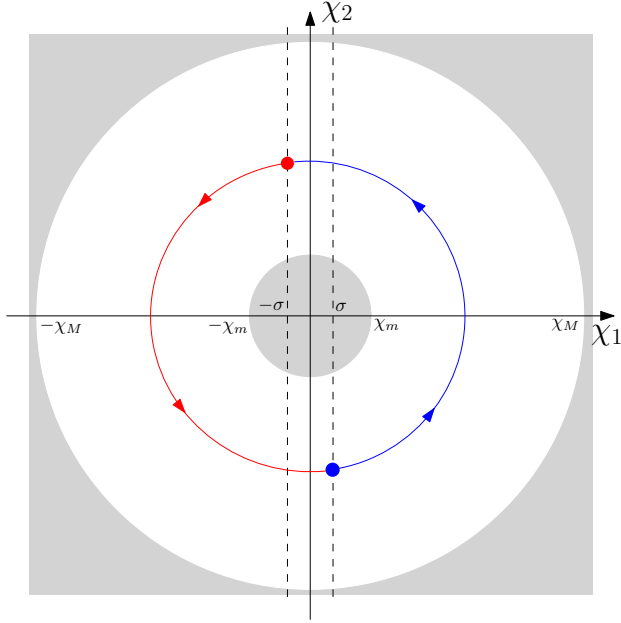
Figure 4: The white doughnut represents the set \mathcal{W} . The red/blue curve is a solution \chi(t, j) where the dots represents jump instants. The solution is blue in regions where \mathfrak{h}(\chi(t, j)) = -1 and is red in regions where \mathfrak{h}(\chi(t, j)) = 1
