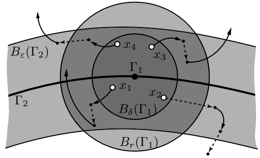
Figure 1: An illustration of local stability of \Gamma_2 near \Gamma_1 . Continuous lines denote flow, while dashed lines denote jumps. All solutions starting sufficiently close to \Gamma_1 remain close to \Gamma_2 so long as they remain in B_r(\Gamma_1) . In the figure, the solution from x_1 remains in B_r(\Gamma_1) and therefore also in B_\varepsilon(\Gamma_2) . The solution from x_2 jumps out of B_r(\Gamma_1) , then jumps out of B_\varepsilon(\Gamma_2) . The solution from x_3 flows out of B_r(\Gamma_1) , then flows out of B_\varepsilon(\Gamma_2) . Finally, the solution from x_4 jumps out of B_r(\Gamma_1) , then flows out of B_\varepsilon(\Gamma_2) .
