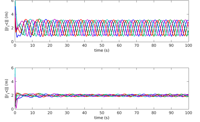
Fig. 8. Evolution of the relative distance of each agent with respect to the target, \|\mathbf{r}_i(t) - \mathbf{c}(t)\| , for a simulation of 5 agents following and encircling the time-varying target \mathbf{c}(t) in a flowfield for two values of parameter \mathbf{K} : \mathbf{K} = \mathbf{I}_2 (top) and \mathbf{K} = 10\mathbf{I}_2 (bottom).
