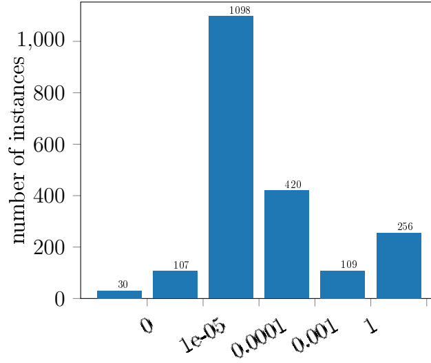
FIGURE 1. Number of instances where the difference of numerical lower bound and exact lower bound lies in the given interval; note that the exact bound sometimes is better.
